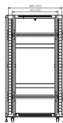
Maximum Mounting Depth
