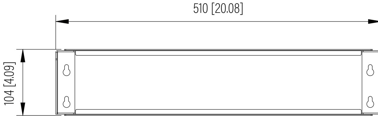
Front View
