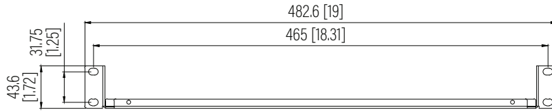
Front View
