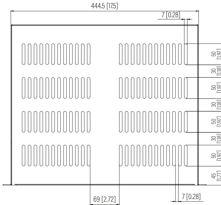
Top View
