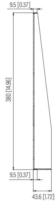
Side View
