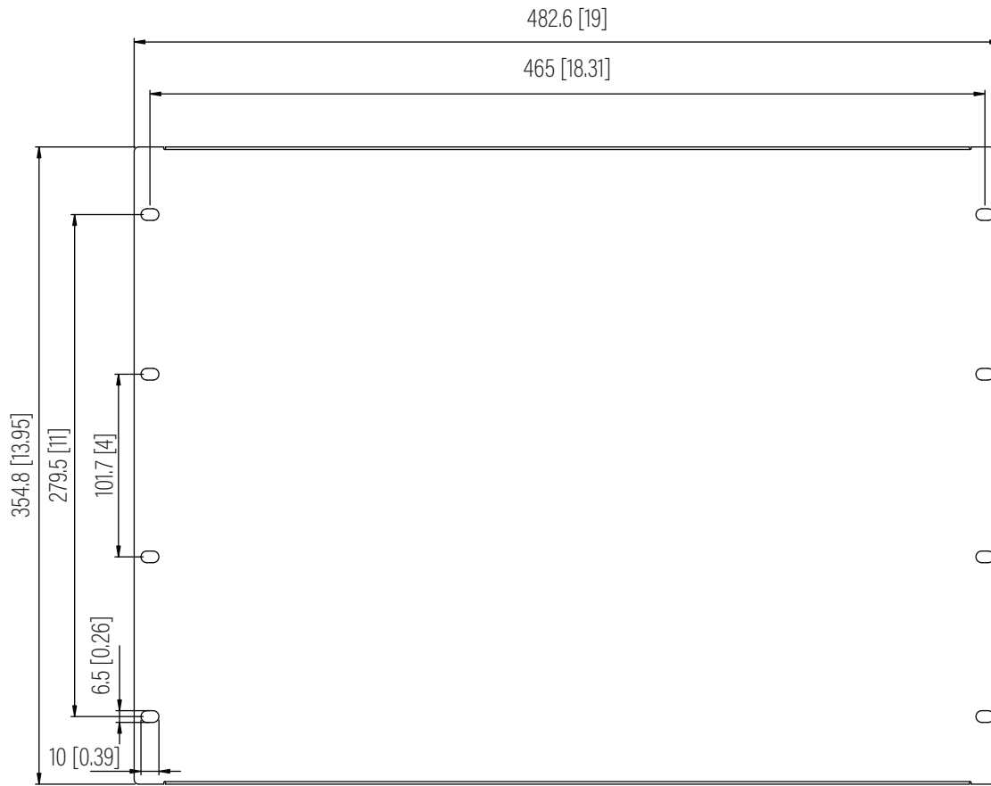
Front View
