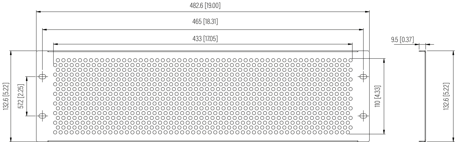
Front View
