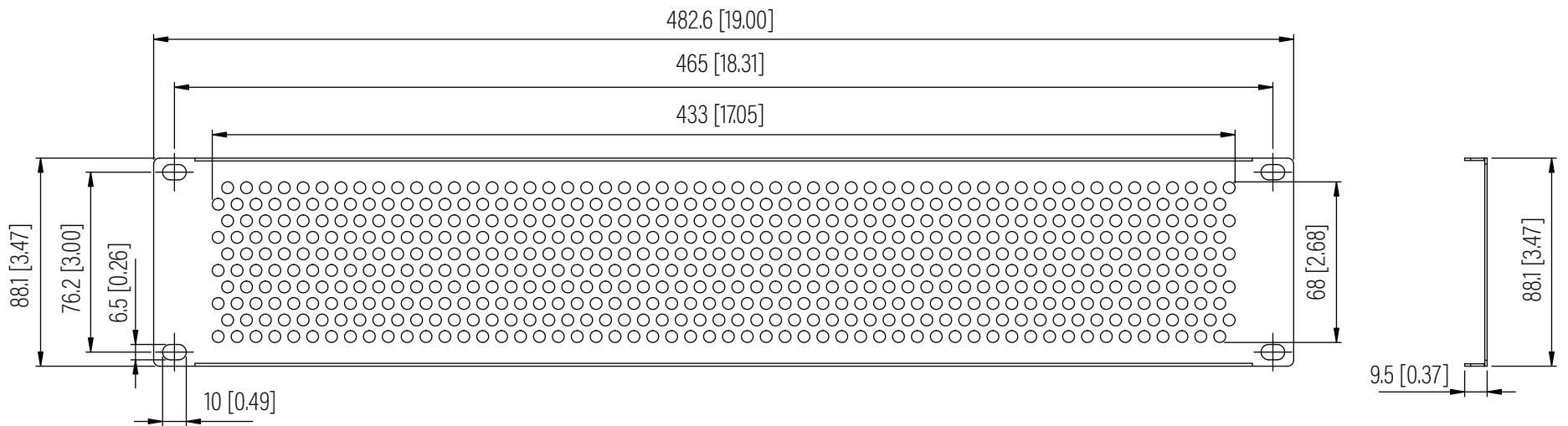
Front View
