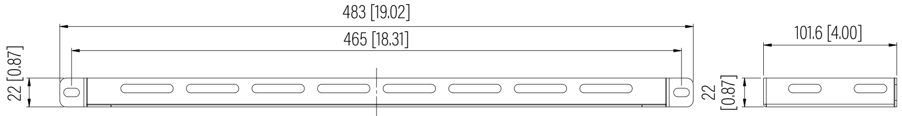
Front View
