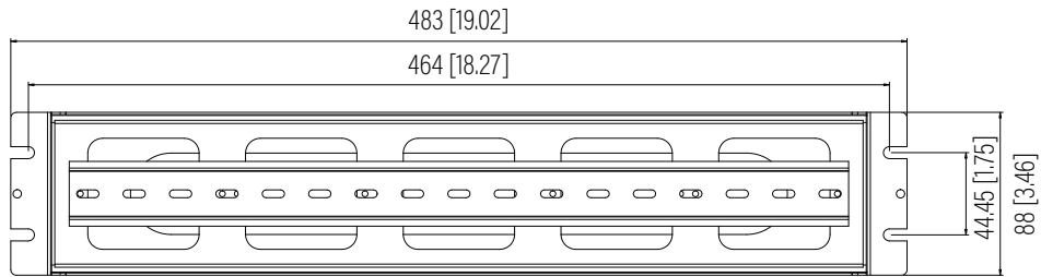
Front View
