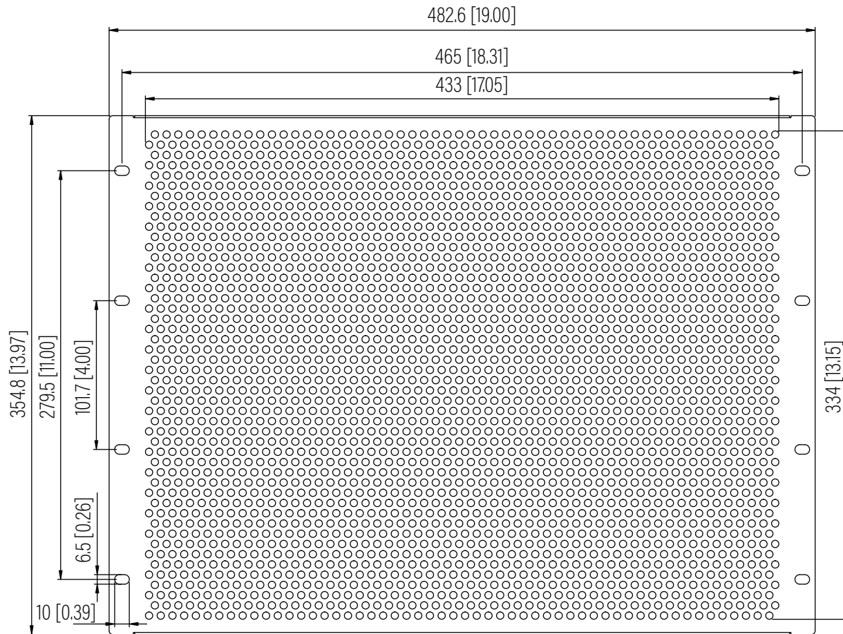
Front View
