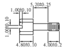
UNC #4-40 Hexscrew
