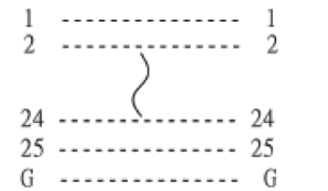
DGC 25 F/F GENDER CHANGER PIN OUT: 25Female
