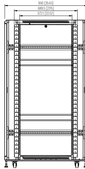
Side View, Factory Default Mounting Depth
