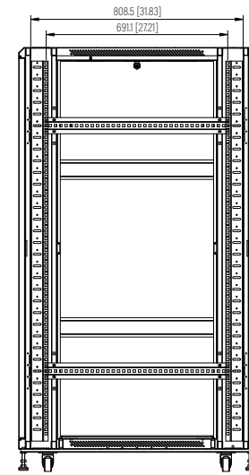
Maximum Mounting Depth
