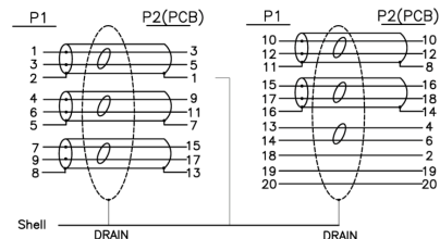
PIN Assignment
