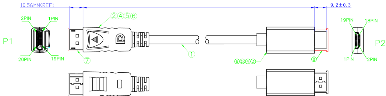
PIN Assignment
