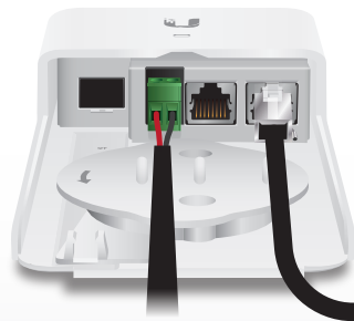
24/50V DC Output 24/50V Power and Data from PoE Adapter or PoE Switch
