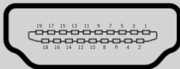
HDMI type A cable pin layout
