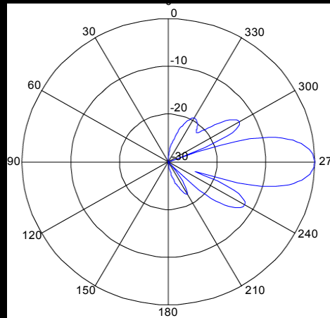
RF Patterns Horizontal Cut, Typ.
